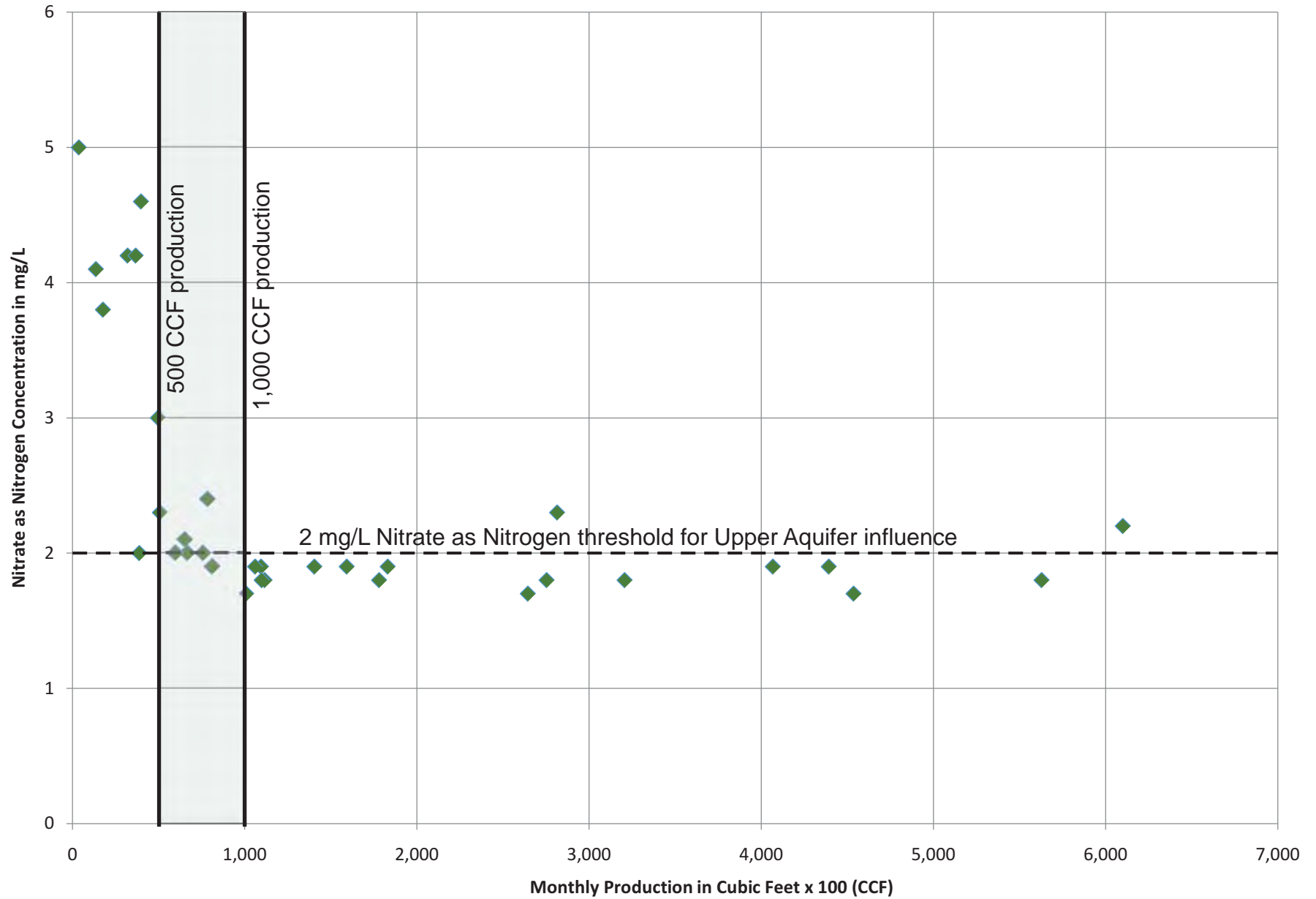
Figure J3 Production vs Nitrate as Nitrogen Metric Well LA10 Purveyor Monitoring Data 2018 Annual Report
