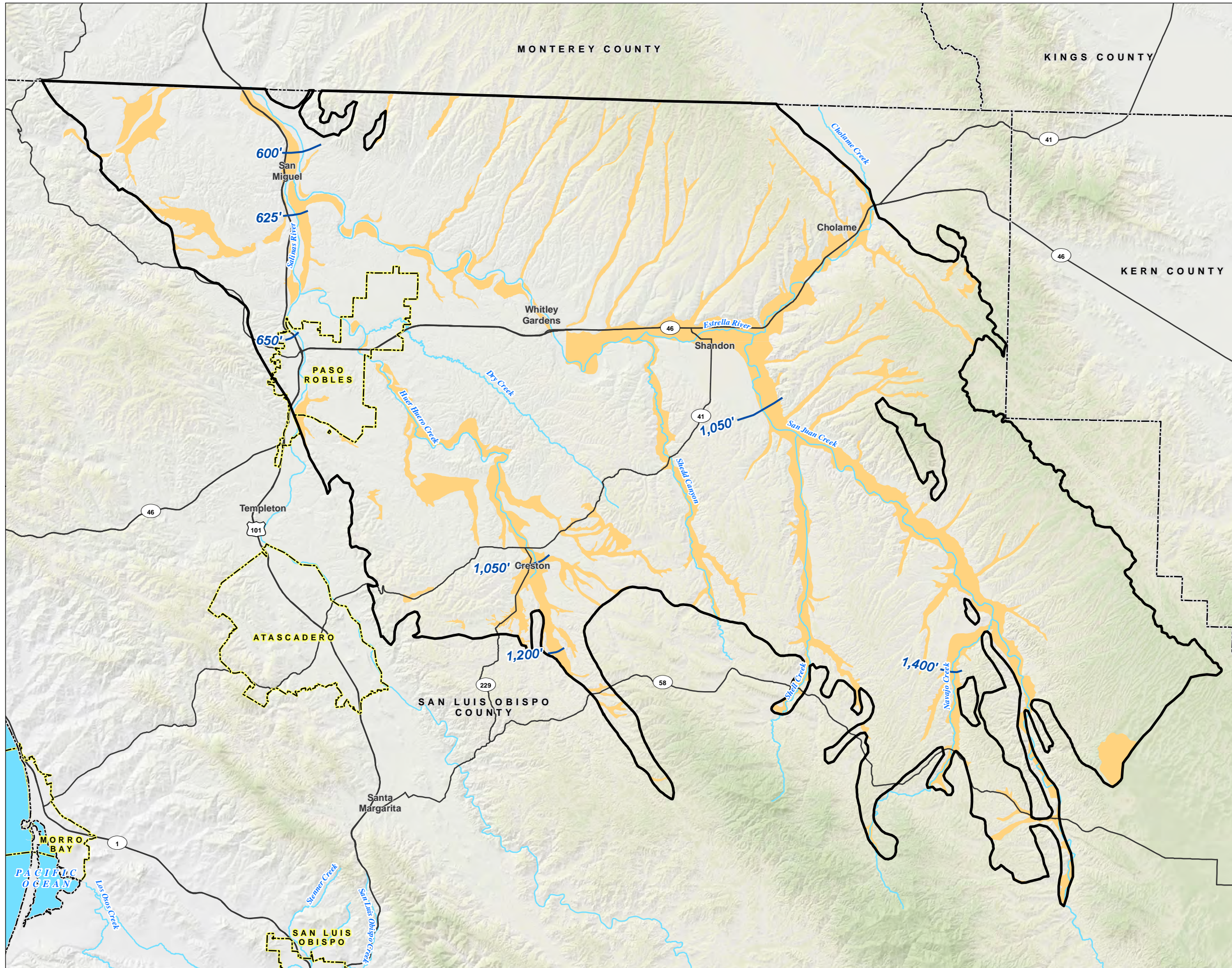
FIGURE 4 Alluvial Aquifer Groundwater Elevation Contours Paso Robles Subbasin First Annual Report
