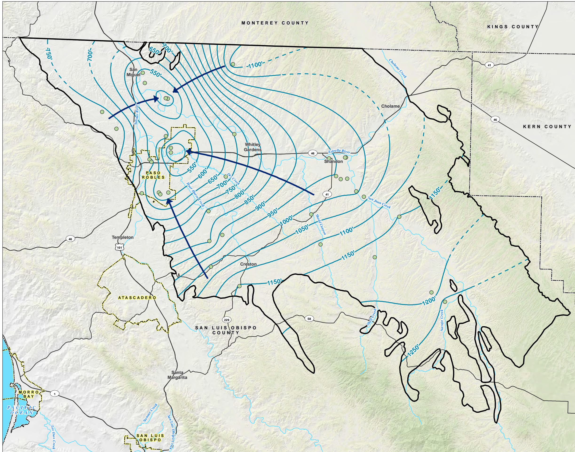
FIGURE 9 Paso Robles Formation Aquifer Fall 2019 Groundwater Elevation Contours Paso Robles Subbasin First Annual Report
