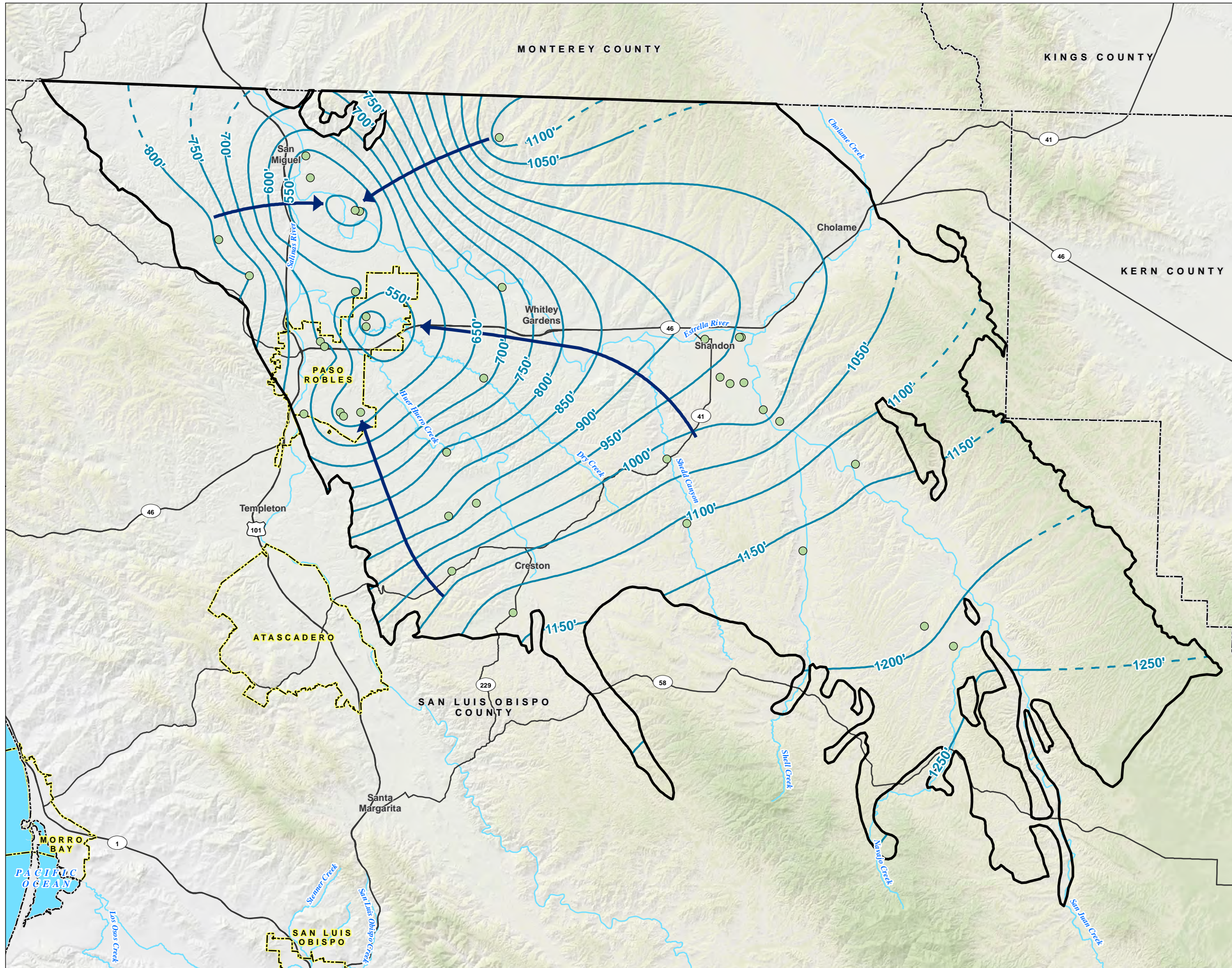
FIGURE 7 Paso Robles Formation Aquifer Fall 2018 Groundwater Elevation Contours Paso Robles Subbasin First Annual Report
