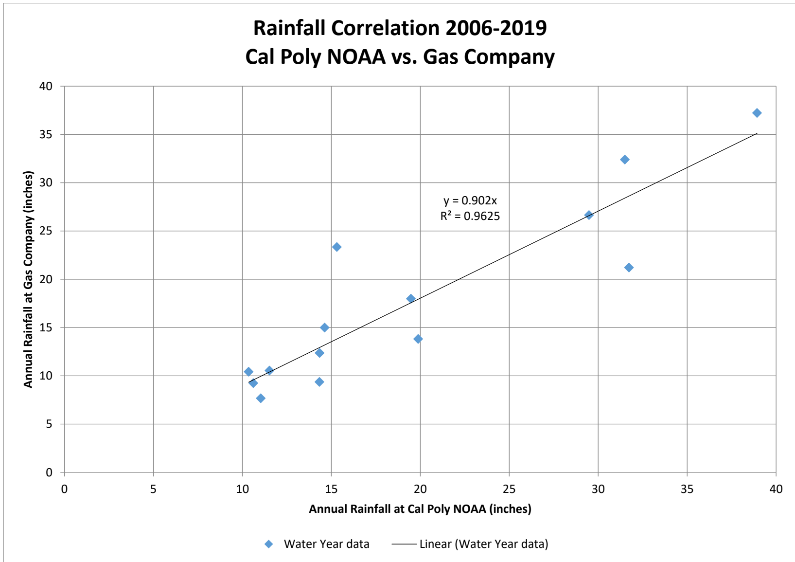
Figure 6-11: Rainfall Correlation Cal Poly vs. Gas Company.
