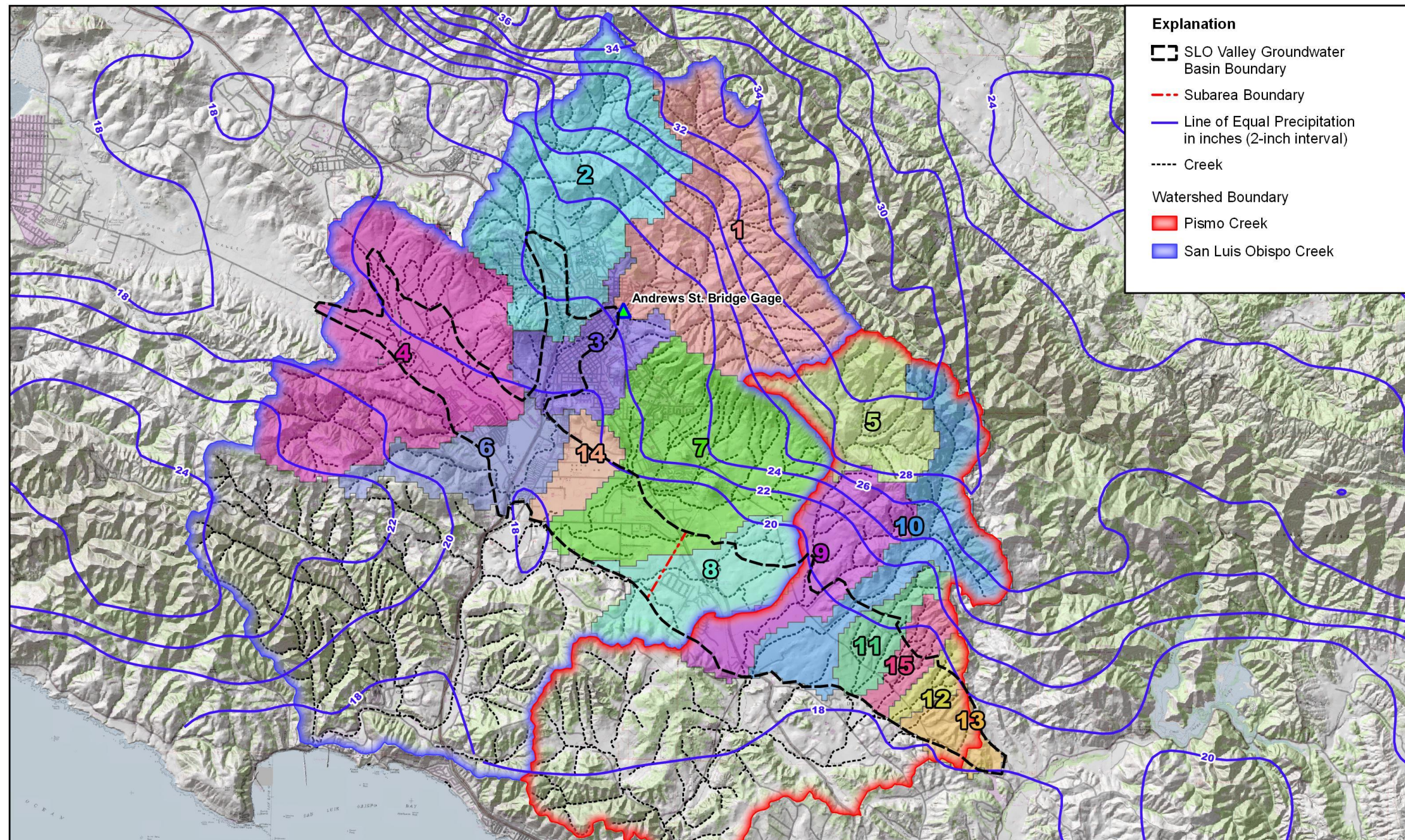
Basin Sub-watershed Areas and Isohyetals Figure 6-13
