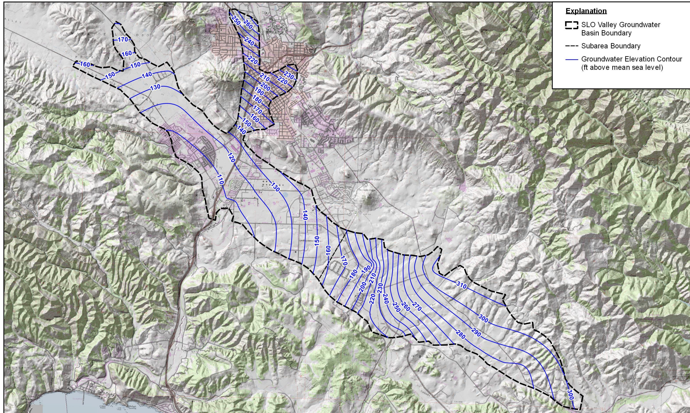
Groundwater Elevation Contours Spring 1986
