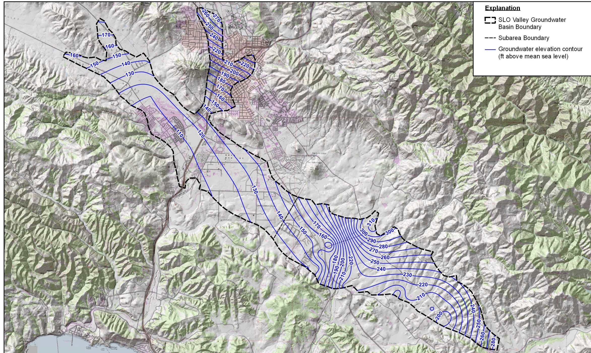
Groundwater Elevation Contours Spring 2019
