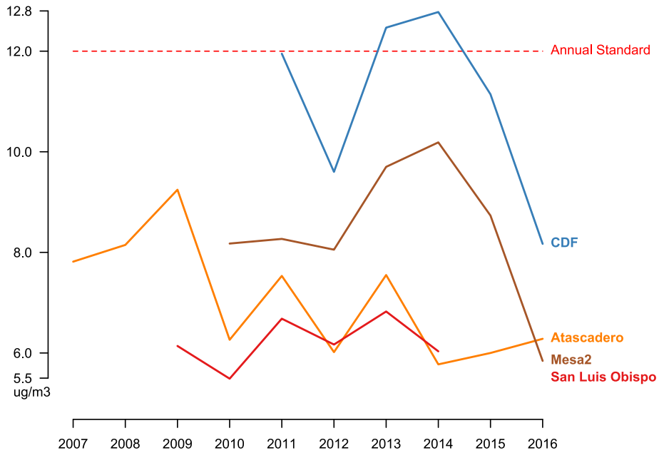
Figure VII-7 – PM 2.5 Annual Averages, 2007-2016
