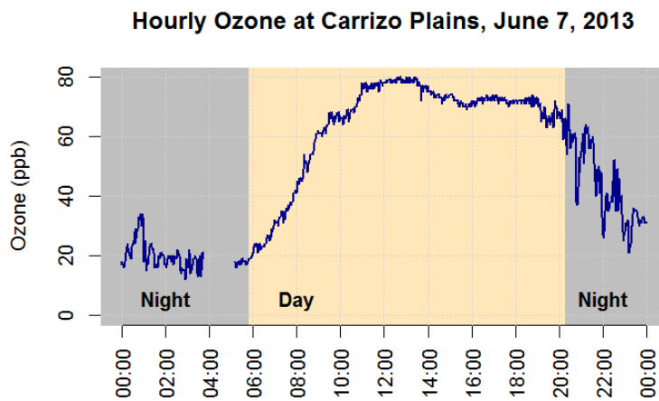
Figure VII-1 – Example of Diurnal Ozone Pattern
