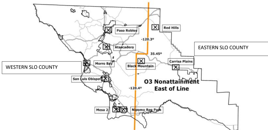
Figure VII-2 – Ozone Nonattainment Area
