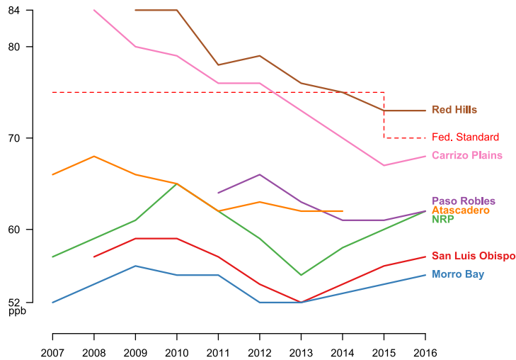
Figure VII-4 – Ozone Design Value Trends, 2007-2016
