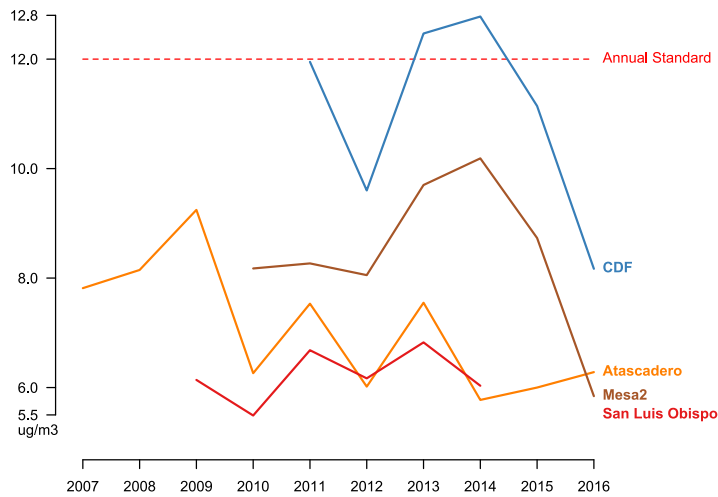
Figure VII-7 – PM 2.5 Annual Averages, 2007-2016
