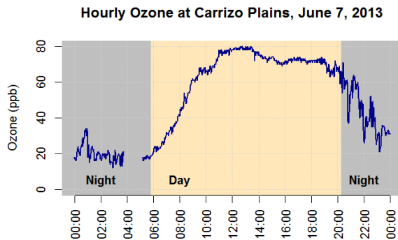
Figure VII-1 – Example of Diurnal Ozone Pattern
