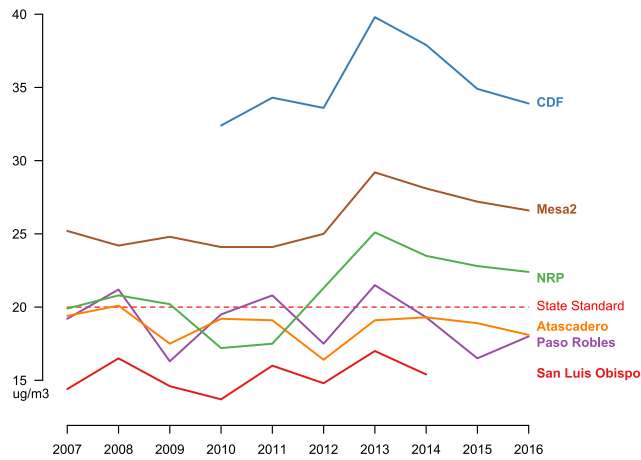
Figure VII-6 – \text{PM}_{10} Annual Average, 2007-2016
