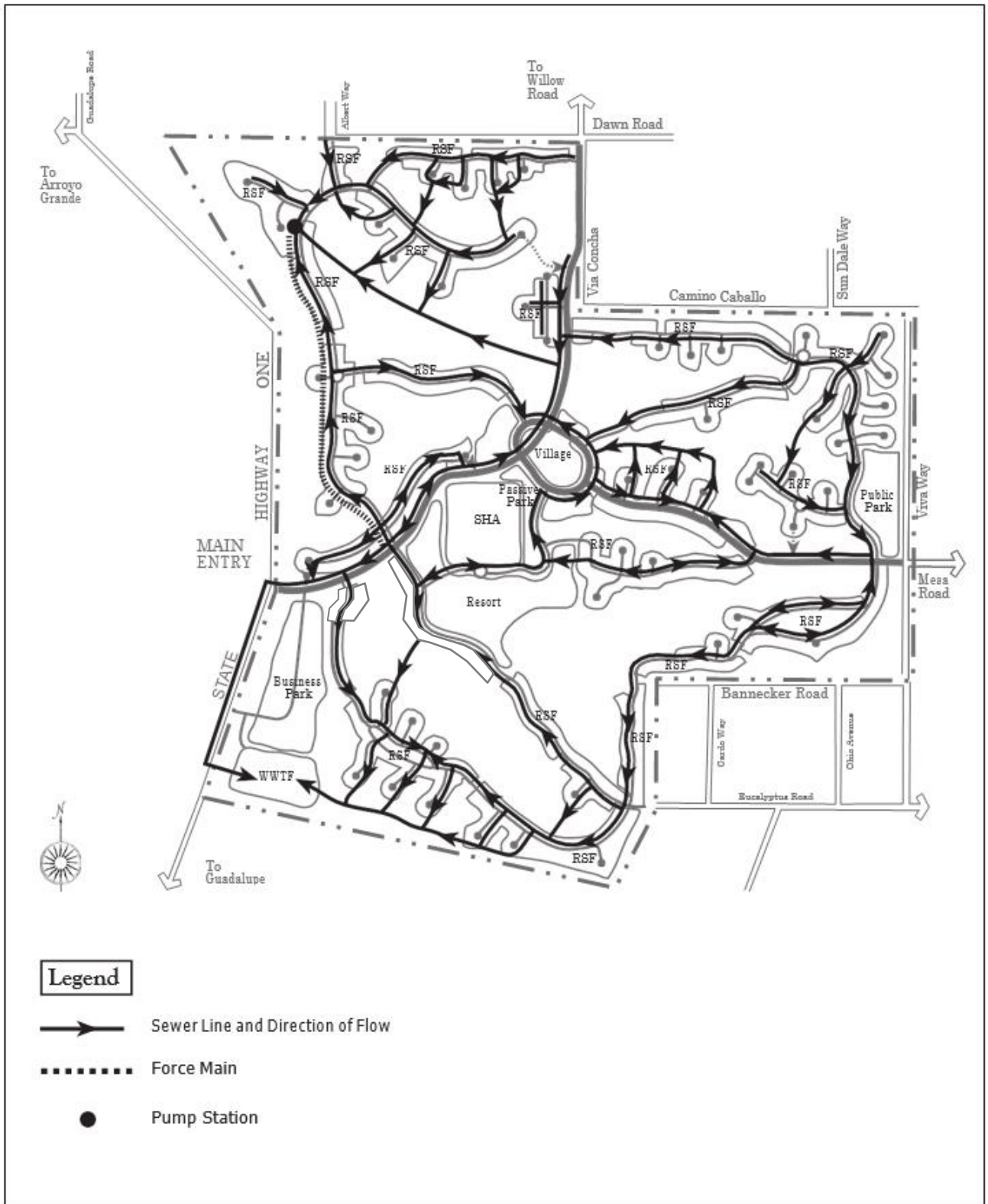
Sanitary Sewer Service Map
