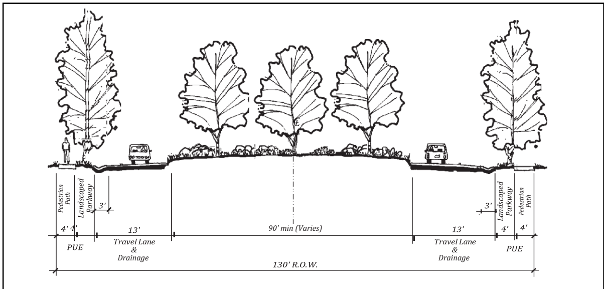
Section H - Roundabout
