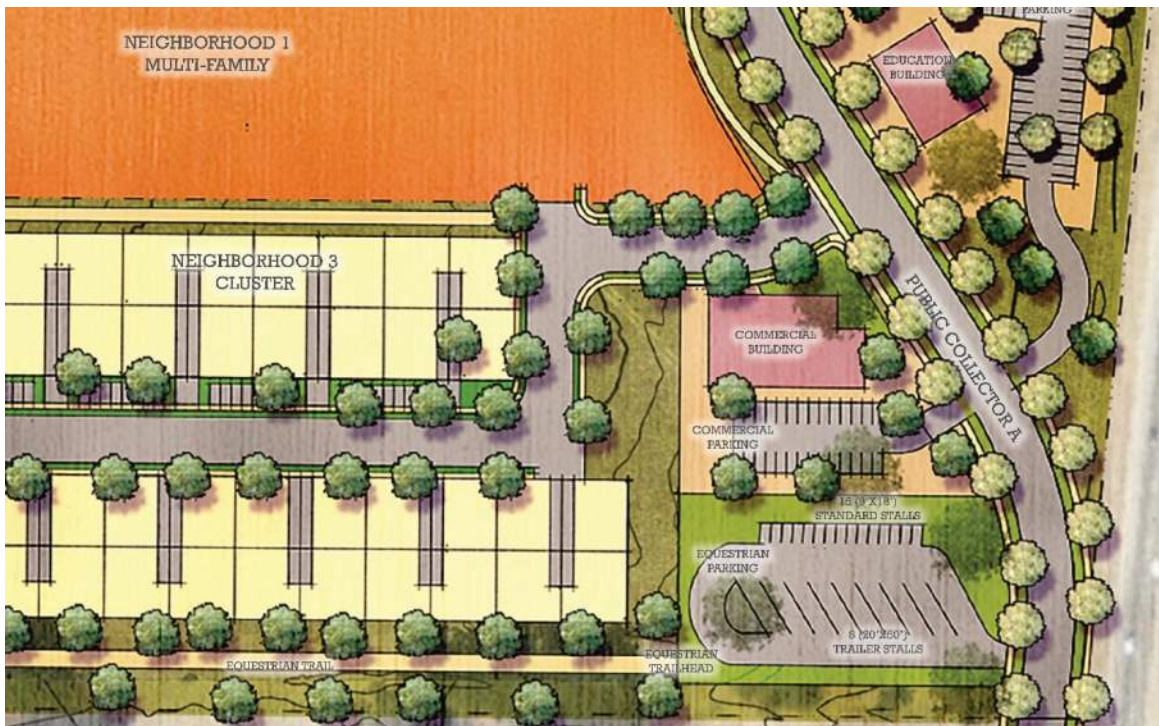
Exhibit 4-18: Equestrian Trailhead Concept
