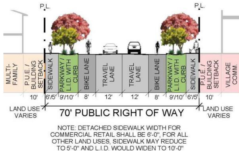
Exhibit 4-4: Collector 'A' Adjacent to Village Commercial
