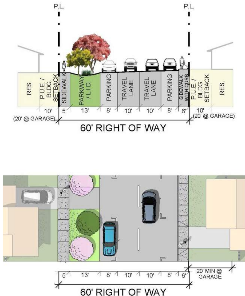
Exhibit 4-13: Single-Family Street, Alternative
