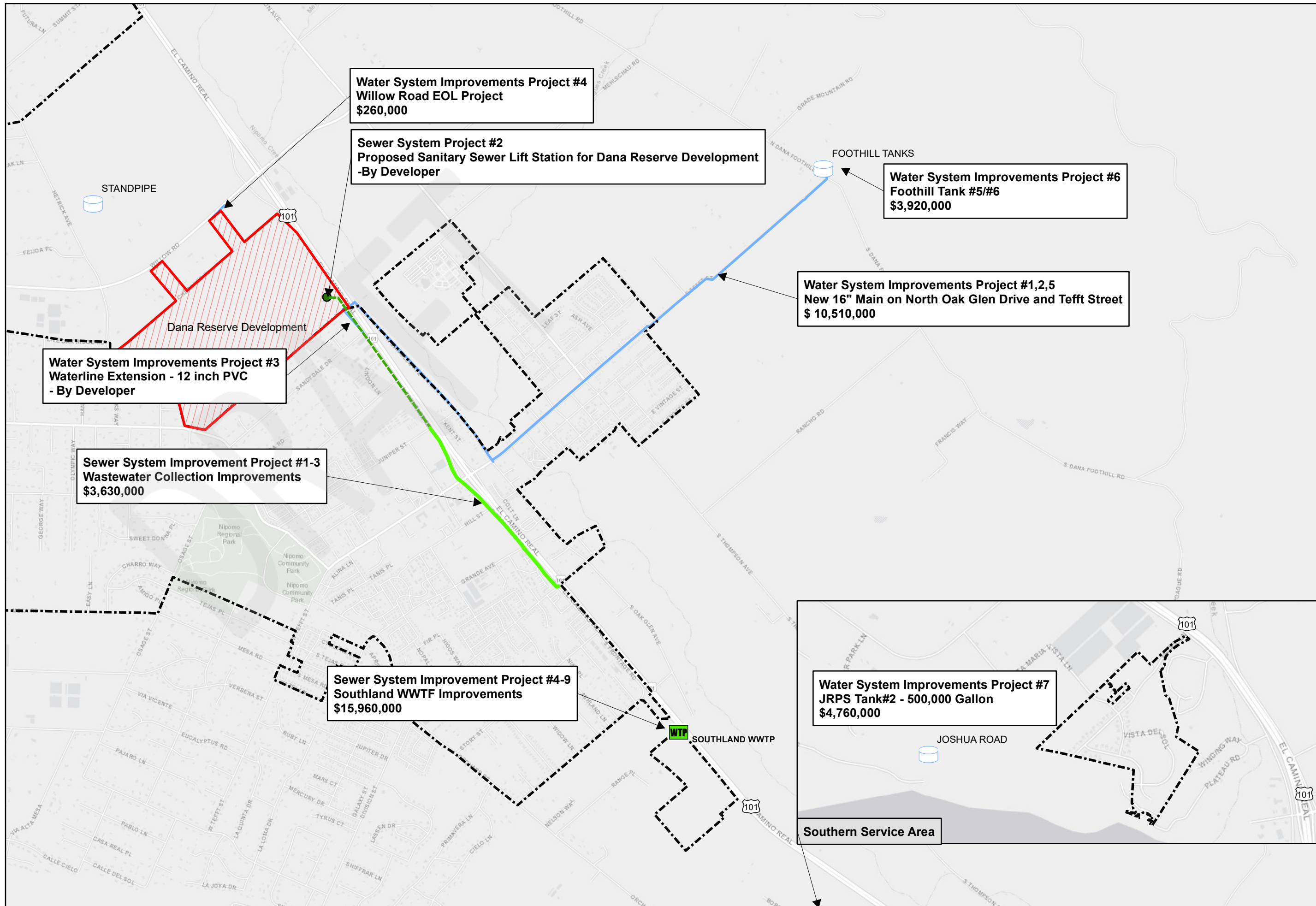
Figure 6-5 Proposed Water and Sewer System Improvements
