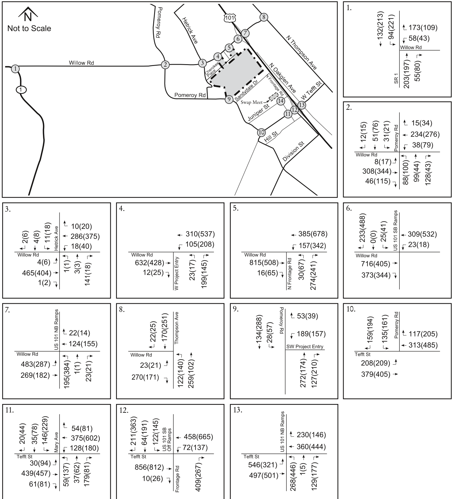
Figure 6: Existing Plus Project Weekday Peak Hour Volumes
