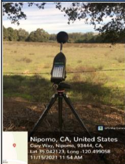
MEASUREMENT LOCATION 3
