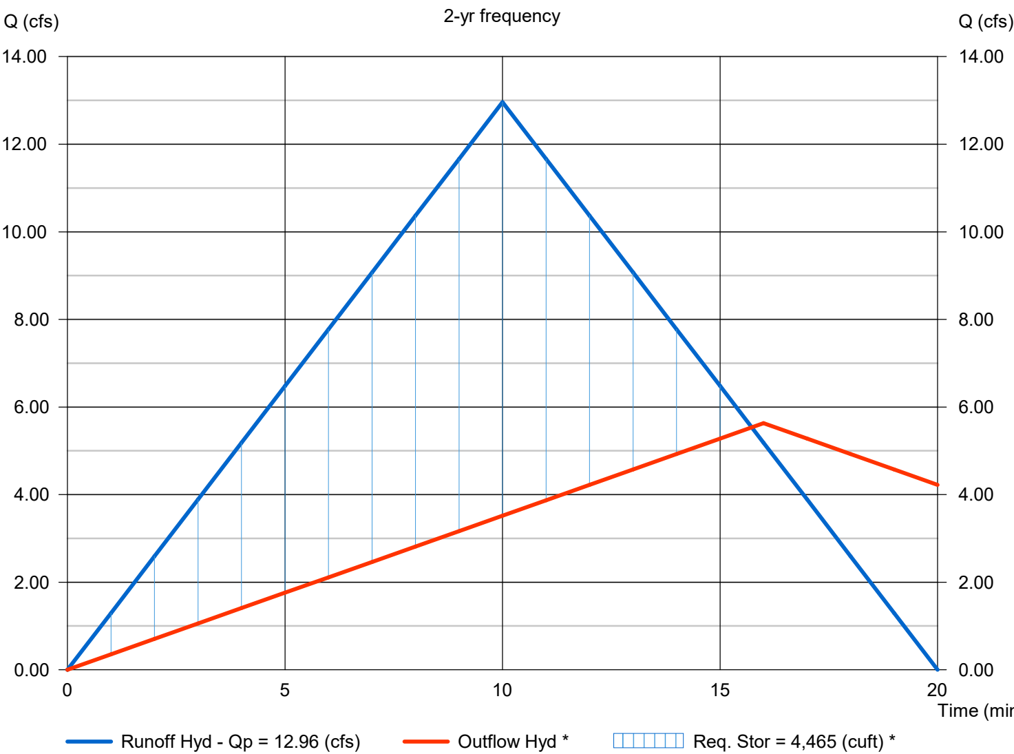
Runoff Hydrograph
