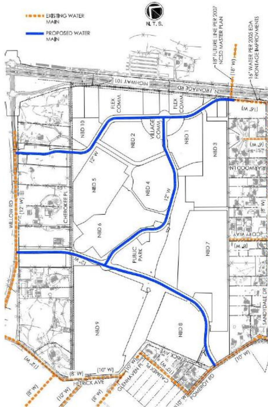
Exhibit 5-1: Proposed Water Backbone Infrastructure
