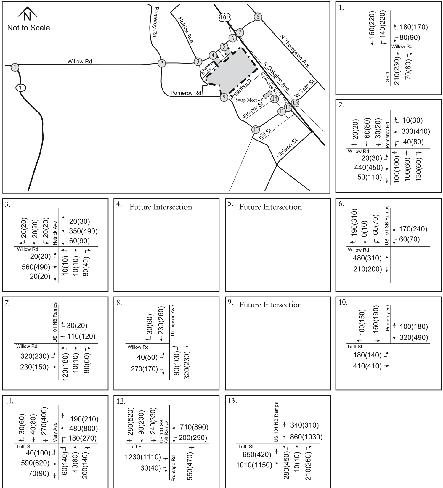
Figure 7: Cumulative Weekday Peak Hour Volumes
