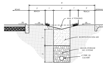
A ROADSIDE INFILTRATION BIOSWALE SCALE 1"=2'
