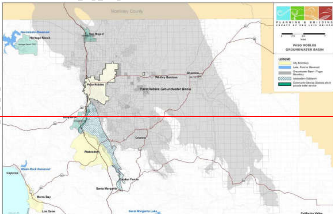
Figure 2-2 – Paso Robles Groundwater Basin Excluding the Atascadero Sub-basin Paso Basin Land Use Management Area
