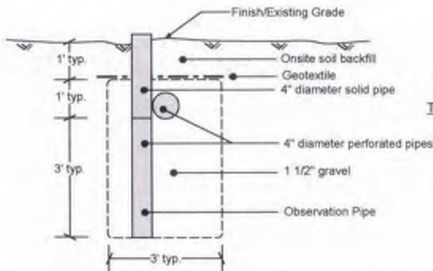
TRENCH PROFILE 1" = 10'H +/- 1" = 5'V +/-
