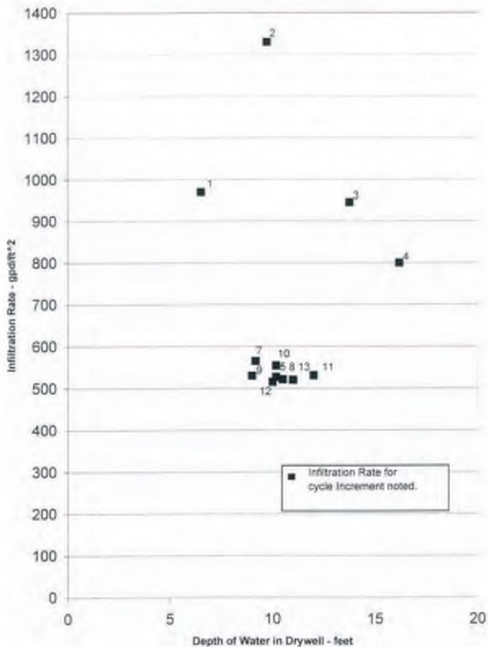
Drywell Infiltration Rate vs. Head in Well
