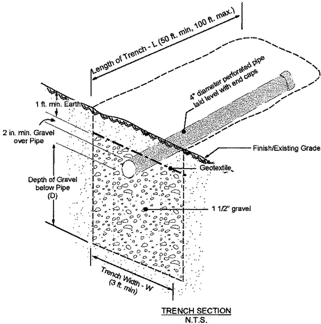
TYPICAL PERCOLATION LINE DETAIL Los Osos Wastewater Project Los Osos, California
