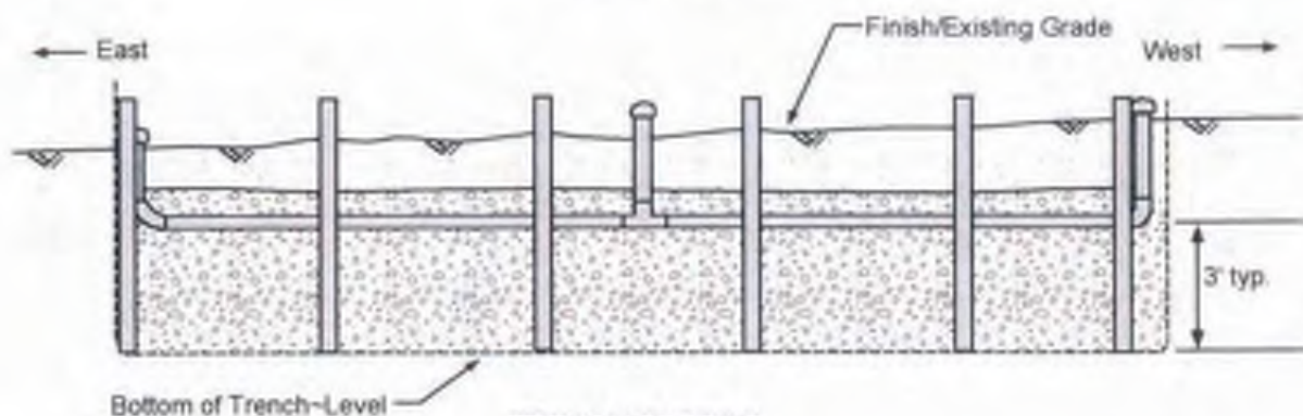
TRENCH PROFILE 1" = 10'H +/- 1" = 5'V +/-
