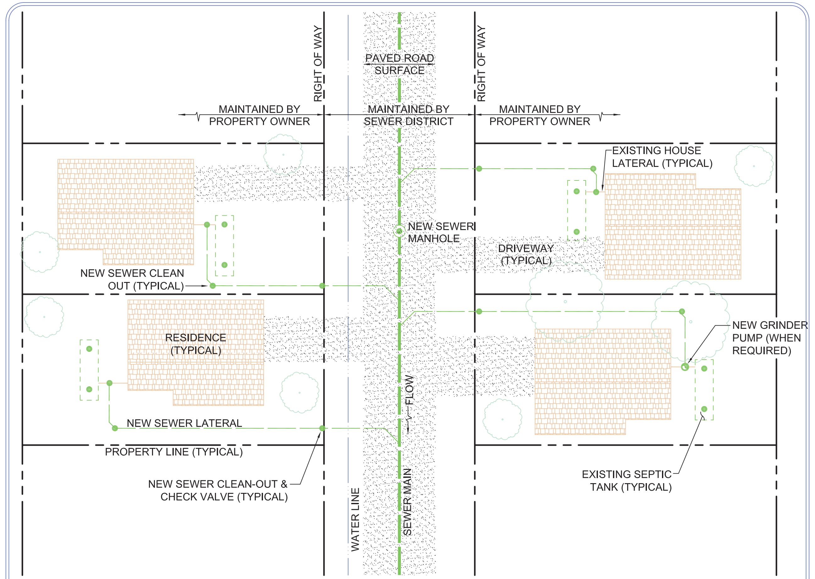
COLLECTION ON-LOT INSTALLATION CONDITIONS
