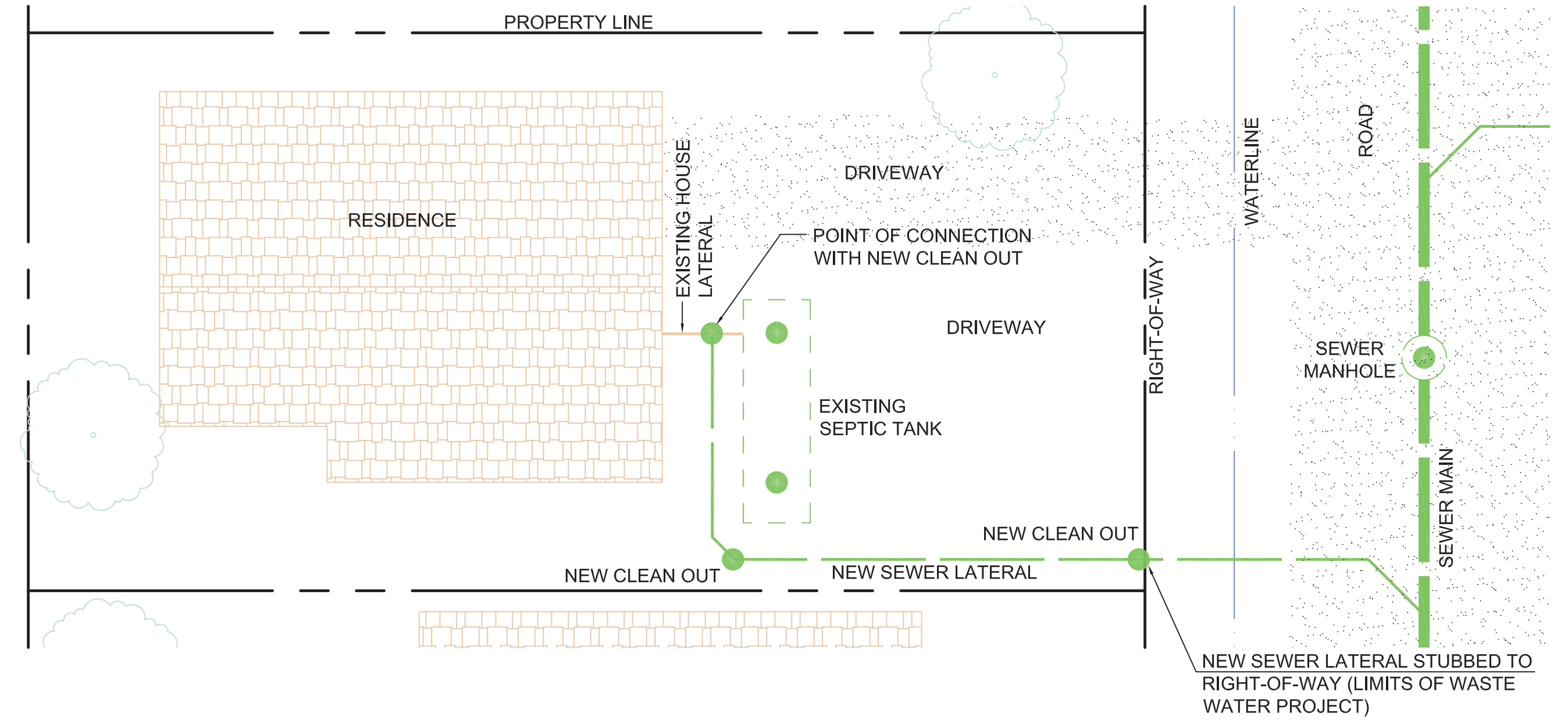
CONDITION 2: SEPTIC TANK LOCATED IN FRONT YARD
