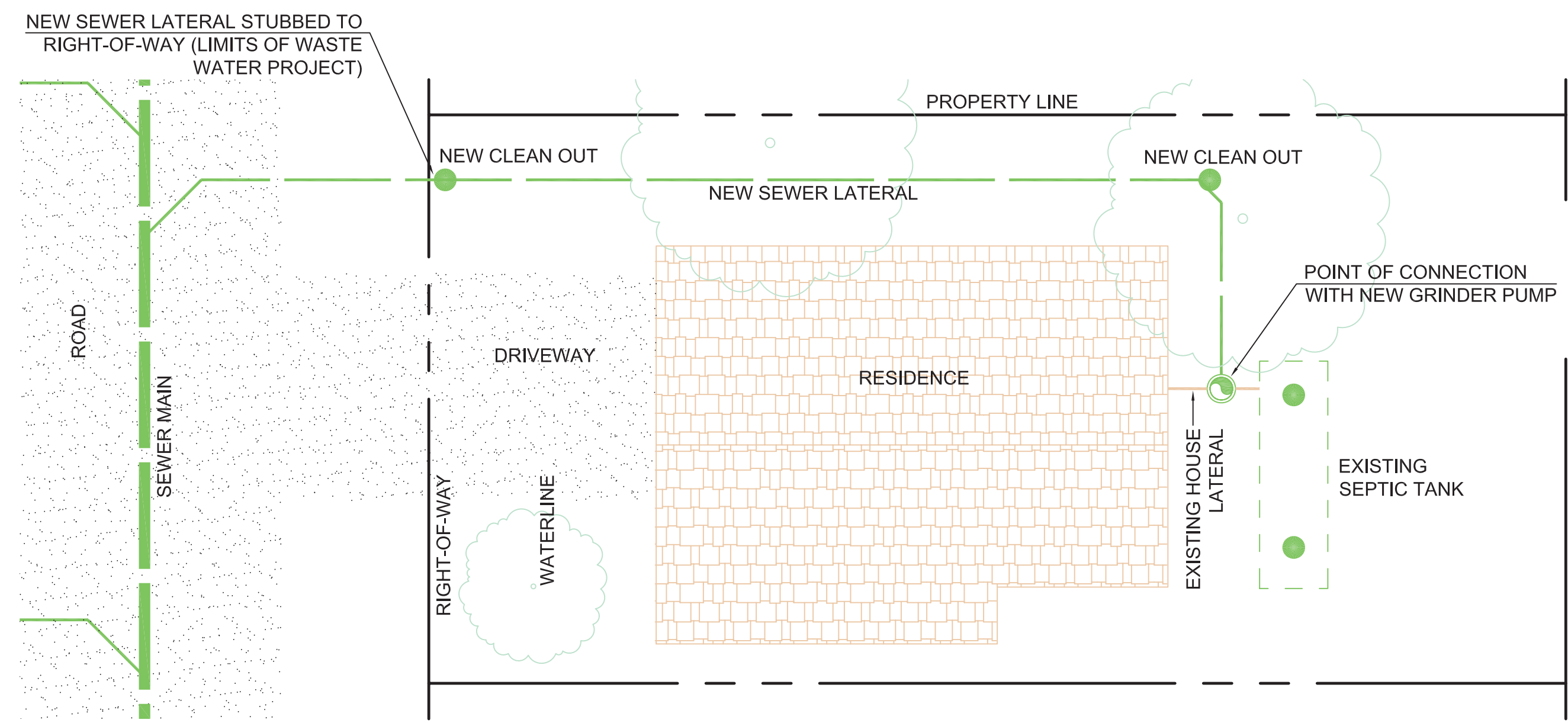
CONDITION 3: SEPTIC TANK LOCATED IN BACK YARD WITH RESTRICTED ACCESS
