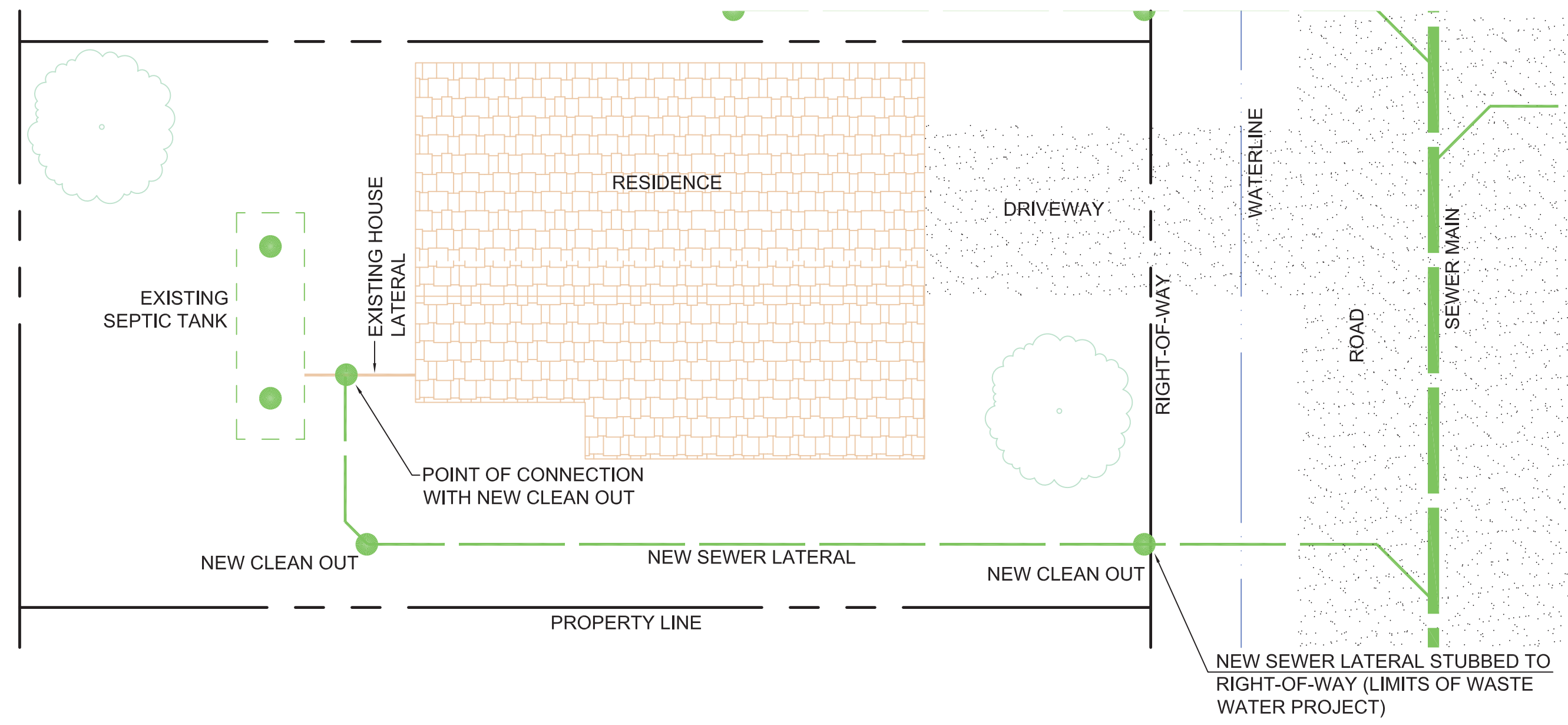
CONDITION 1: SEPTIC TANK LOCATED IN BACK YARD
