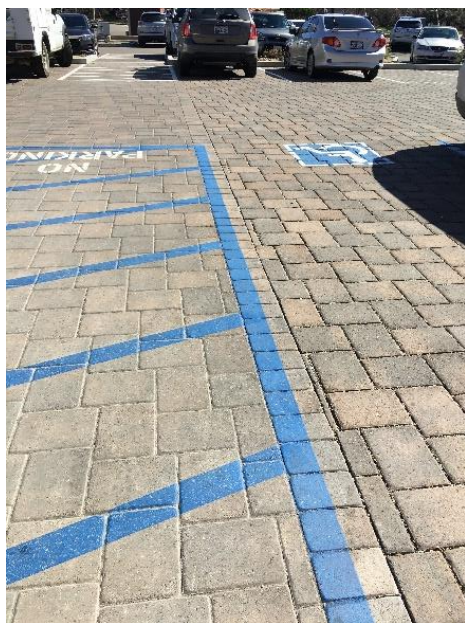
Figure 1918: Transition from pervious interlocking pavers to traditional pavers in ADA path of travel.
