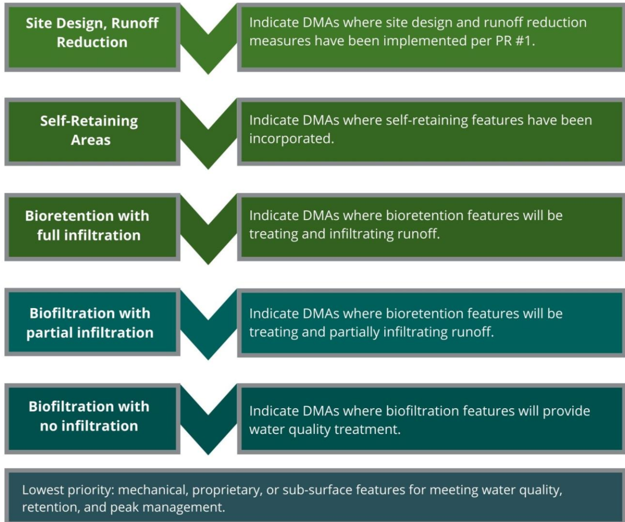
Figure 14: Low impact development prioritization framework.
