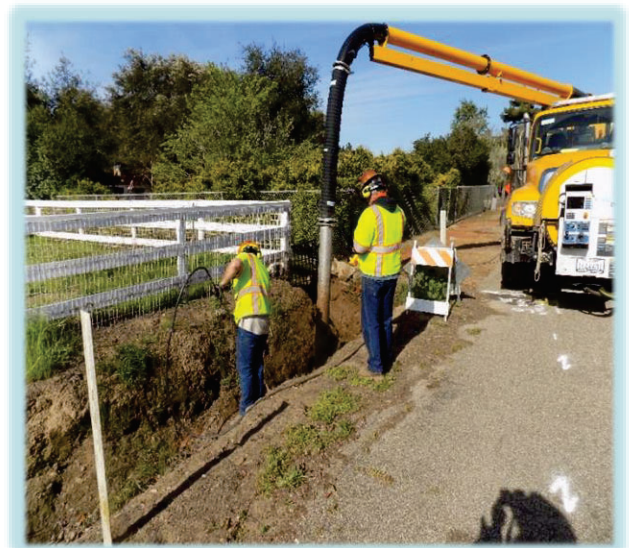
CULVERT MAINTENANCE – PABLO LANE, NIPOMO
